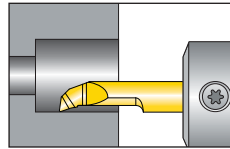
Boring
